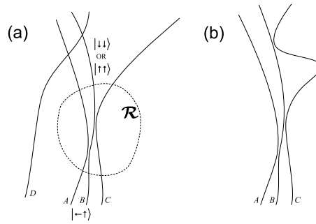
Figure 1. Spacetime diagrams. (a) Particles A, B, C interact and become entangled. A and B subsequently interact with other systems D , but not with C or any system influenced by C (but see section 5.3). The resulting evolution is non-unitary, placing A and B in one of |\downarrow\downarrow\rangle or |\uparrow\uparrow\rangle (before their further possible interactions with D ). (b) Particles A, B, C interact and become entangled, and then C subsequently becomes disentangled with the others. This evolution is unitary and part of some larger event.
