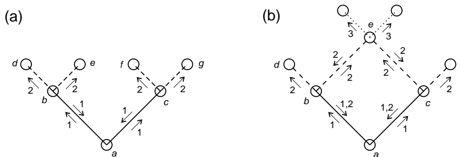
Figure 2. Spacetime diagrams, showing a sketch of a transactional-type mechanism for detecting spacetime loops and thus deciding what type(s) of event can happen. An emitter a emits offer waves (OW, retarded) to absorbers b and c , which in turn emit second-order OWs. (a) No absorber receives two 2nd-order OWs, so no 2nd-order CWs return to b and c , and these emit only 1st-order CWs to a . (b) An absorber e receives two 2nd-order OWs. It generates a 3rd-order OW and 2nd order CWs to b and c . The 2nd-order OWs are not fully absorbed, so b and c pass both 1st and 2nd order CWs to a .
