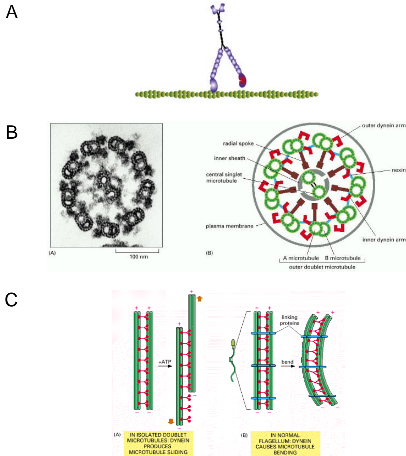
Figure 2-2 (A): Myosin V walks with \sim 36 nm steps. A Myosin V walking with one leg labeled with fluorophore shows \sim 72 nm steps, which suggests a hand-over-hand mechanism. Adapted from
