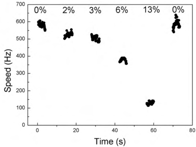
Figure 6-8: Chimeric motor speed with 0.35 \mu\text{m} beads in different viscosity by adding Ficoll, 85 mM [\text{Na}^+]_{\text{ex}} and pH 7. The speeds of each concentration were measured for 5 s. In the end, the medium is exchanged to Ficoll-free sodium motility buffer.
