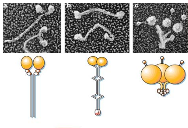
Figure 2-1: Linear molecular motors. (a) Myosin II; (b) kinesin; (c) ciliary dynein. Top row shows electron micrographs of quick-frozen individual molecules. Bottom row shows the cartoon drawing of these motors. Motor domains are in orange. Figure is adapted from [Schliwa, 2003].
