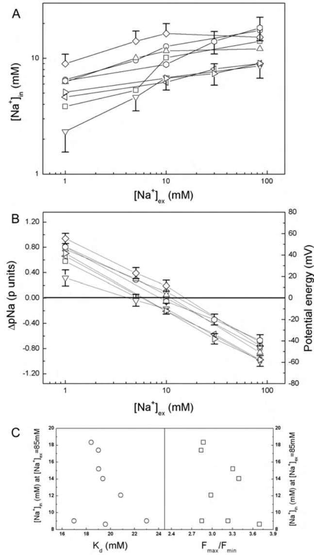
Figure 4-9: [Na]_{in} and \Delta pNa vs. [Na]_{ex} . (A) [Na^+]_{in} vs [Na^+]_{ex} for 8 individual cells expressing the chimeric flagellar motor. (B) The same data as in (A), plotted as \Delta pNa vs [Na^+]_{ex} . (C) Scatter plots of fitted parameters from Equation 4-1, K_d (left) and F_{max}/F_{min} (right), vs [Na^+]_{in} at [Na^+]_{ex} = 85 mM, for the same 8 cells. There were no strong correlations between calibration parameters and [Na^+]_{in} . The standard deviations of K_d , F_{max}/F_{min} , and [Na^+]_{in} were 9.1 %, 9.9 %, and 29.9 % of the mean values respectively. Error bars in (A) and (B) are the same as in Figure 4-8 (A) and (B) respectively.
