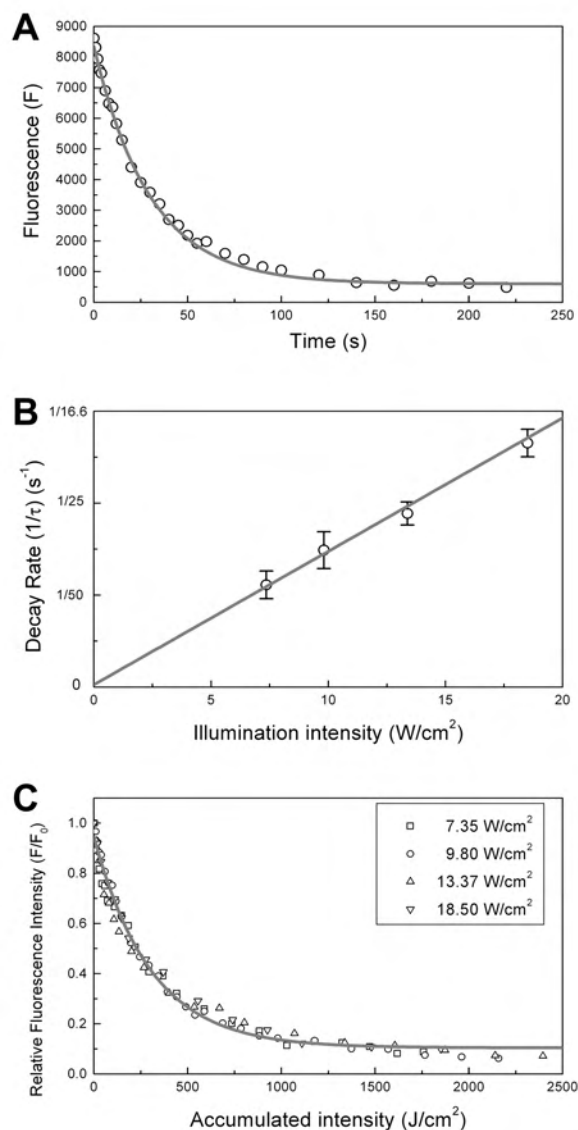
Figure 4-4: Photobleaching of Sodium Green. (A) Fluorescence intensity of a single loaded cell as a function of time during continuous illumination at an intensity of 9.8 \text{ W/cm}^2 , exposure time 1 second. The curve is fitted as exponential decay with a time constant of 30 \pm 0.75 \text{ s} . (B) Photobleaching decay rates as a function of illumination intensity (mean and S.D. of five cells at each intensity). The rates are proportional to intensity as expected for photobleaching (gray line). (C) A combined decay curve for data at different intensities. Photobleaching can be described as F(x) = F_0 \exp(-x/x_0) , where x is the accumulated laser exposure.
