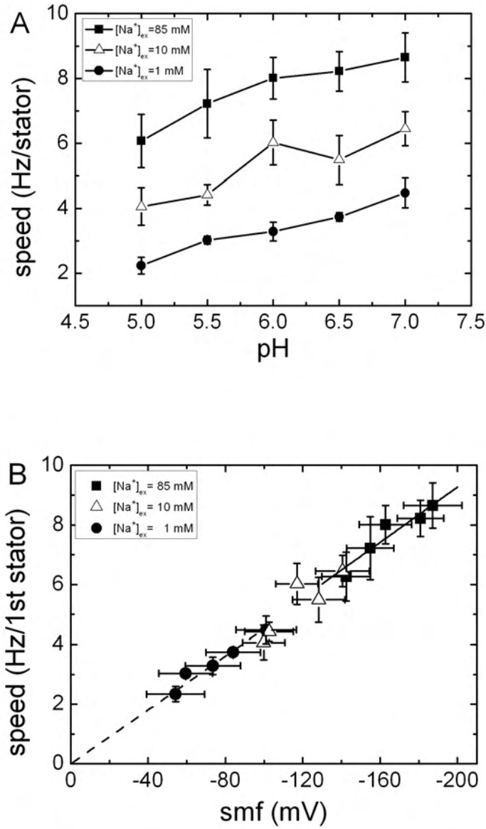
Figure 6-11: Motor speed in high load with 1 \mu m beads. (A) Average motor speed of chimeric motors driving 1 \mu m beads, versus pH_{ex} for different [Na^+]_{ex} . (B) Speed versus smf for pH_{ex} = 7.0, 6.5, 6.0, 5.5, 5.0 and [Na^+]_{ex} = 1, 10, 85 mM. smf values in different media are from Figure 5-10. Linear fits are constrained to the origin for data at 1 mM (dashed lines) and 85 mM (solid lines) [Na^+]_{ex} . Fitted slopes for 1 mM and 85 mM [Na^+]_{ex} respectively are -0.045 \pm 0.001 Hz/stator/mV and -0.046 \pm 0.001 Hz/stator/mV.
