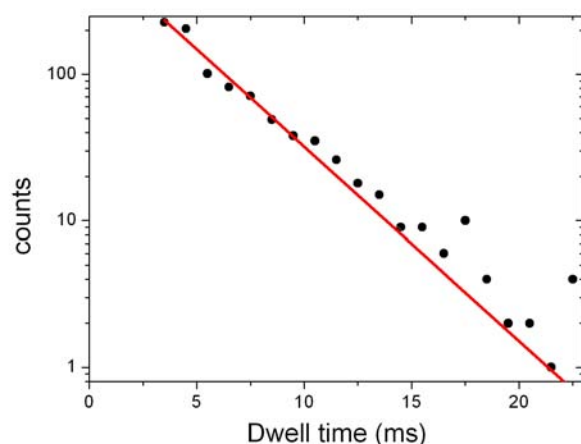
Figure 6-17: Dwell time distribution. The dwell time distribution of the same data trace in Figure 6-15. The dwell time distribution can be fitted with single exponential decay with exponent t_0 = 3.27 \pm 0.1 ms.
