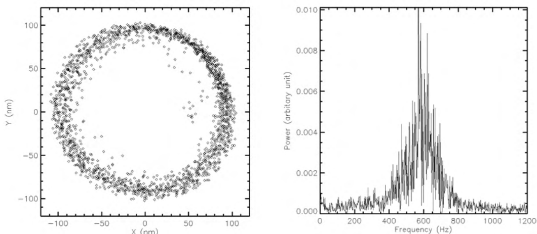
Figure 3-5: Motor speed measurement. A 0.2 \mu\text{m} bead attached to the truncated flagellar filament of YS34 cells with fully-induced PomA/PotB stators. (A) QPD xy data sampled at 10k Hz and (B) raw complex power spectrum with peak \sim 600 Hz.
