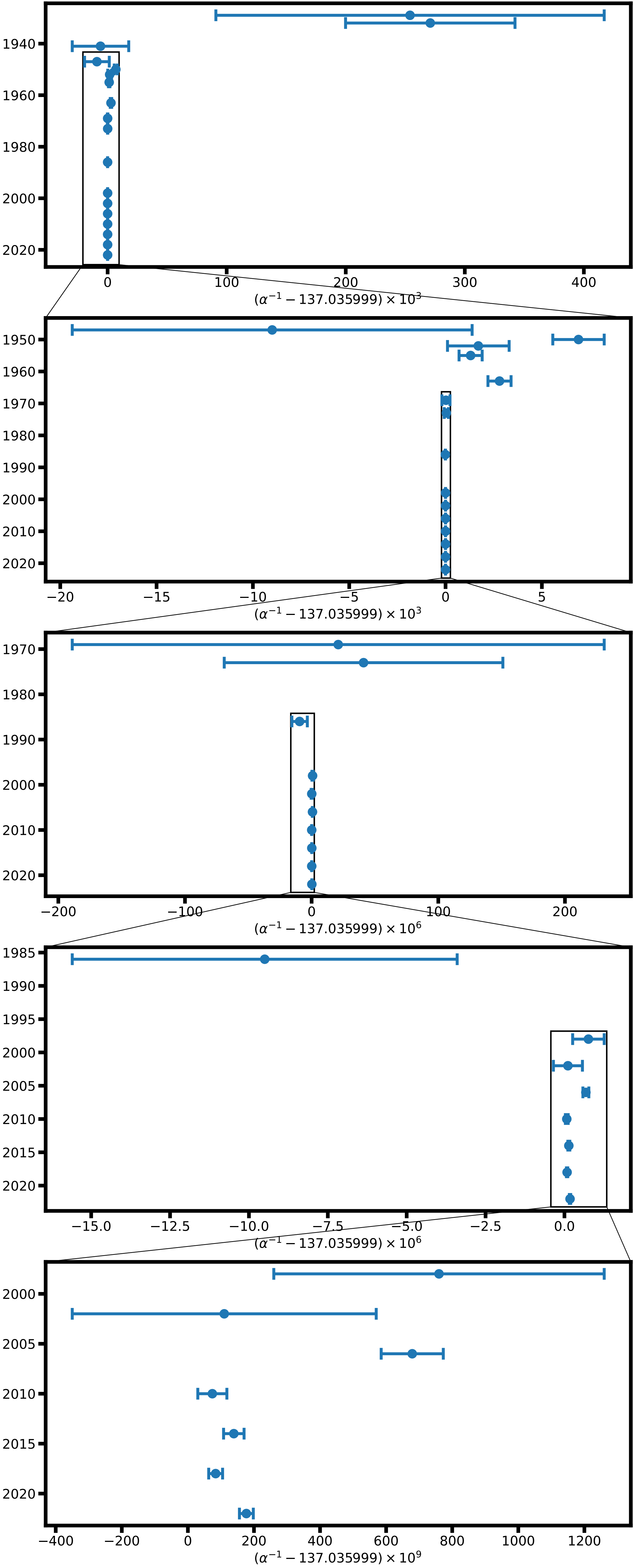
Recommended values for \alpha^{-1}
